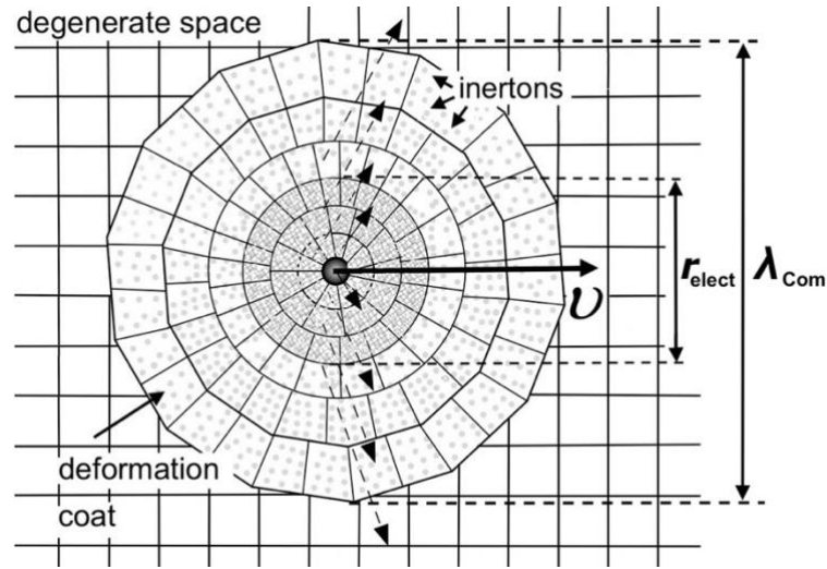
Figure 1. Moving particle in the tessellattice (degenerate space). The deformation coat shields the particle from the degenerate tessellattice. r_{\text{elect}} depicts the size of the electrically polarised sub-coat (in the case of the electron, it is Thomson's classical electron radius; \lambda_{\text{Com}} illustrates the deformation sub-coat induced by the particle mass (it is definitely the Compton wavelength of the particle). The moving particle manifests itself as a wave, covering the environment with spatial excitations – inertons.
